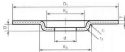
Cut off wheel with depressed center
