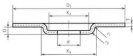
Grinding wheel with depressed center
